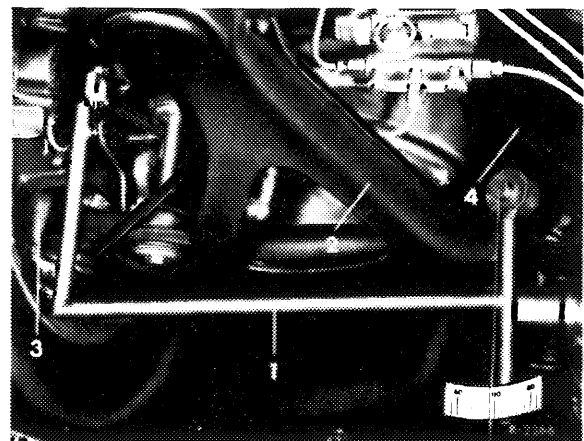
Check position of wishbone arms on model 100
