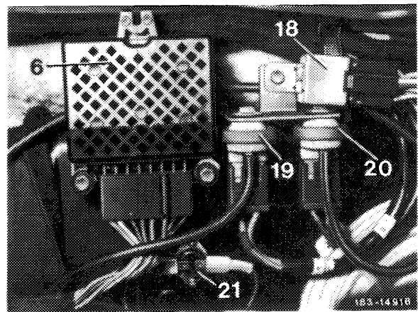
6 Amplifier a 8-point plug connection
